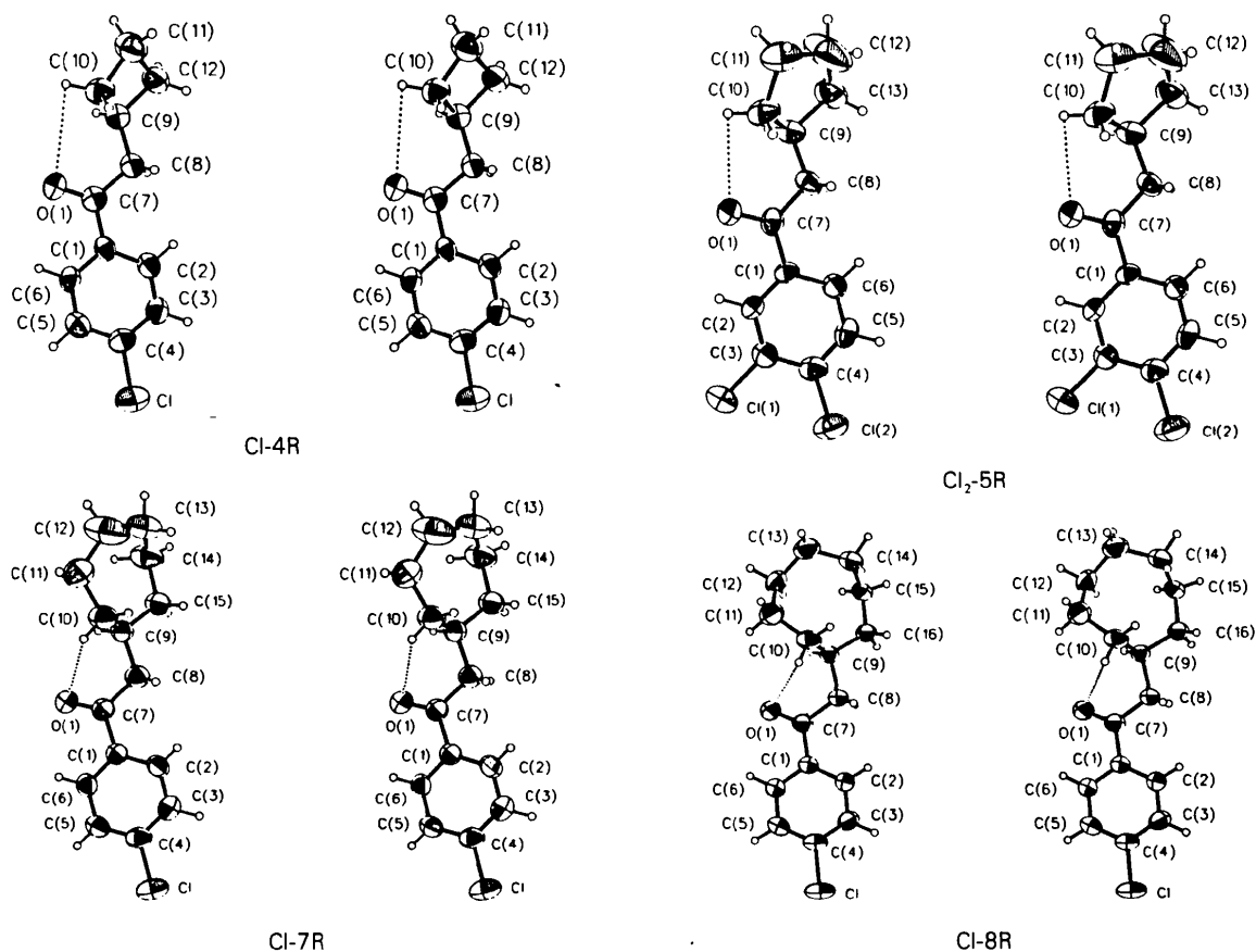
Fig. 5. Stereoviews of the molecules of Cl-4R, Cl 2 -5R (unprimed molecule only), Cl-7R, and Cl-8R. For Cl-4R, the molecule shown is the enantiomorph of that listed in Table 3; the crystals are racemic. Dotted lines indicate H-abstraction pathways.
